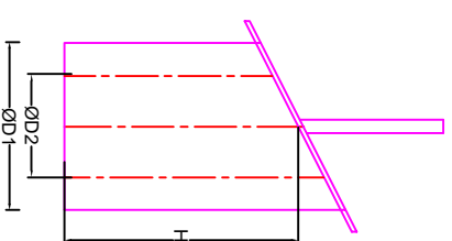
FOR-SIZE-300 to 500 NB-STRAINER WITH 2 BASKETS
